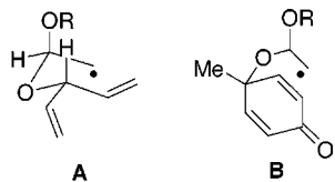
Figure 1. Model for the stereochemical outcome of radical cyclizations starting from 1 (A) and 5 (B).
